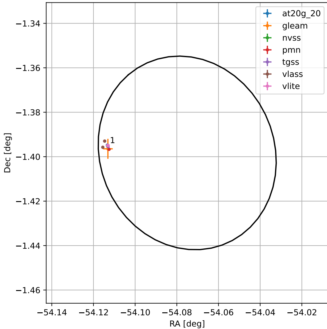
4FGL J2023.6-0123
