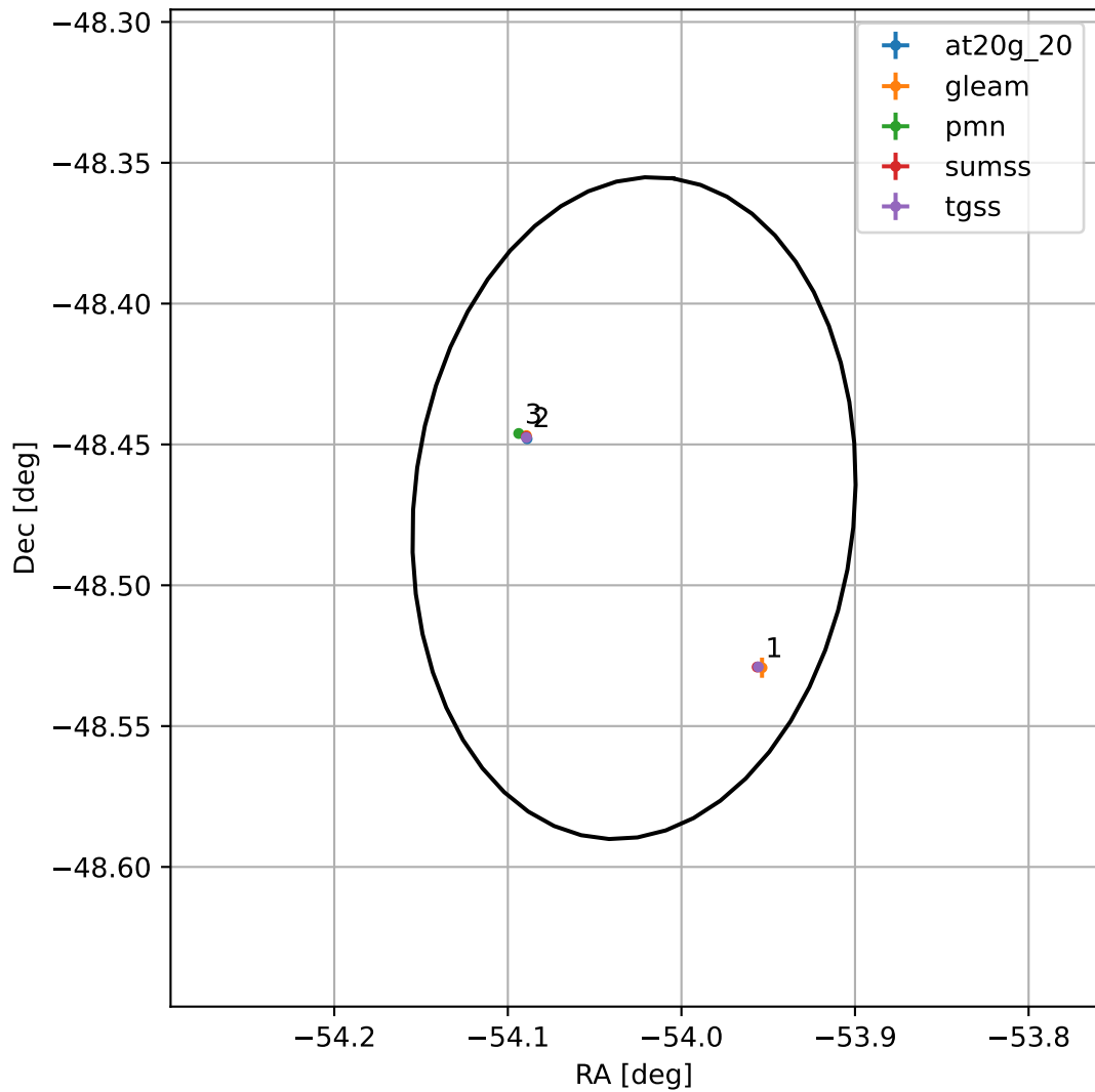
4FGL J2023.8-4828
