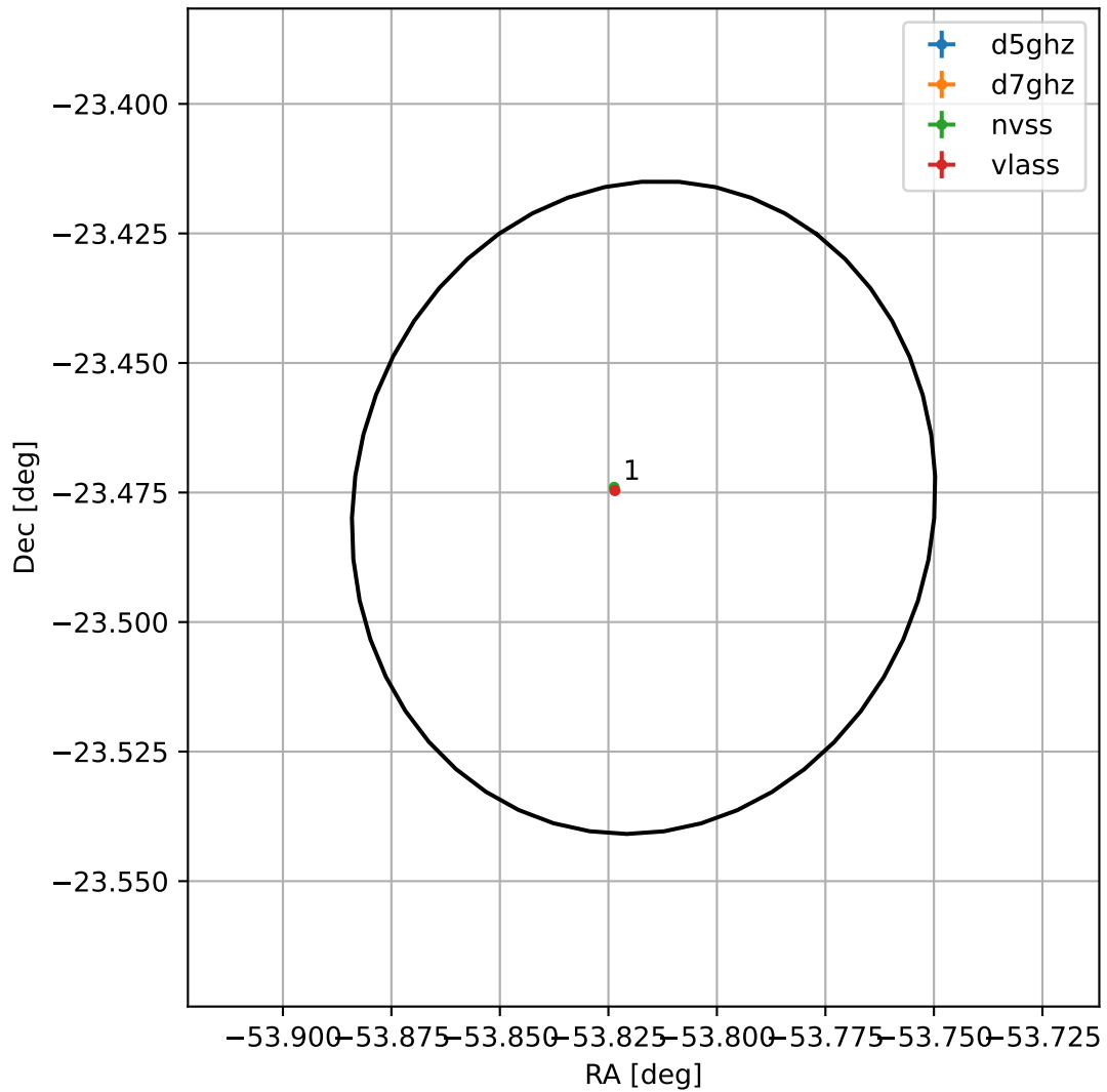
4FGL J2024.7-2328
