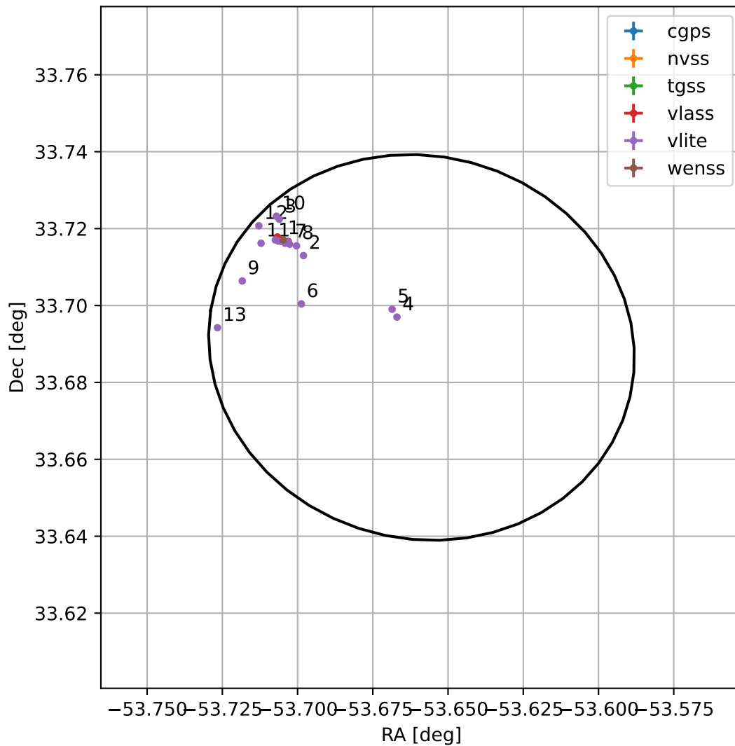
4FGL J2025.3+3341
