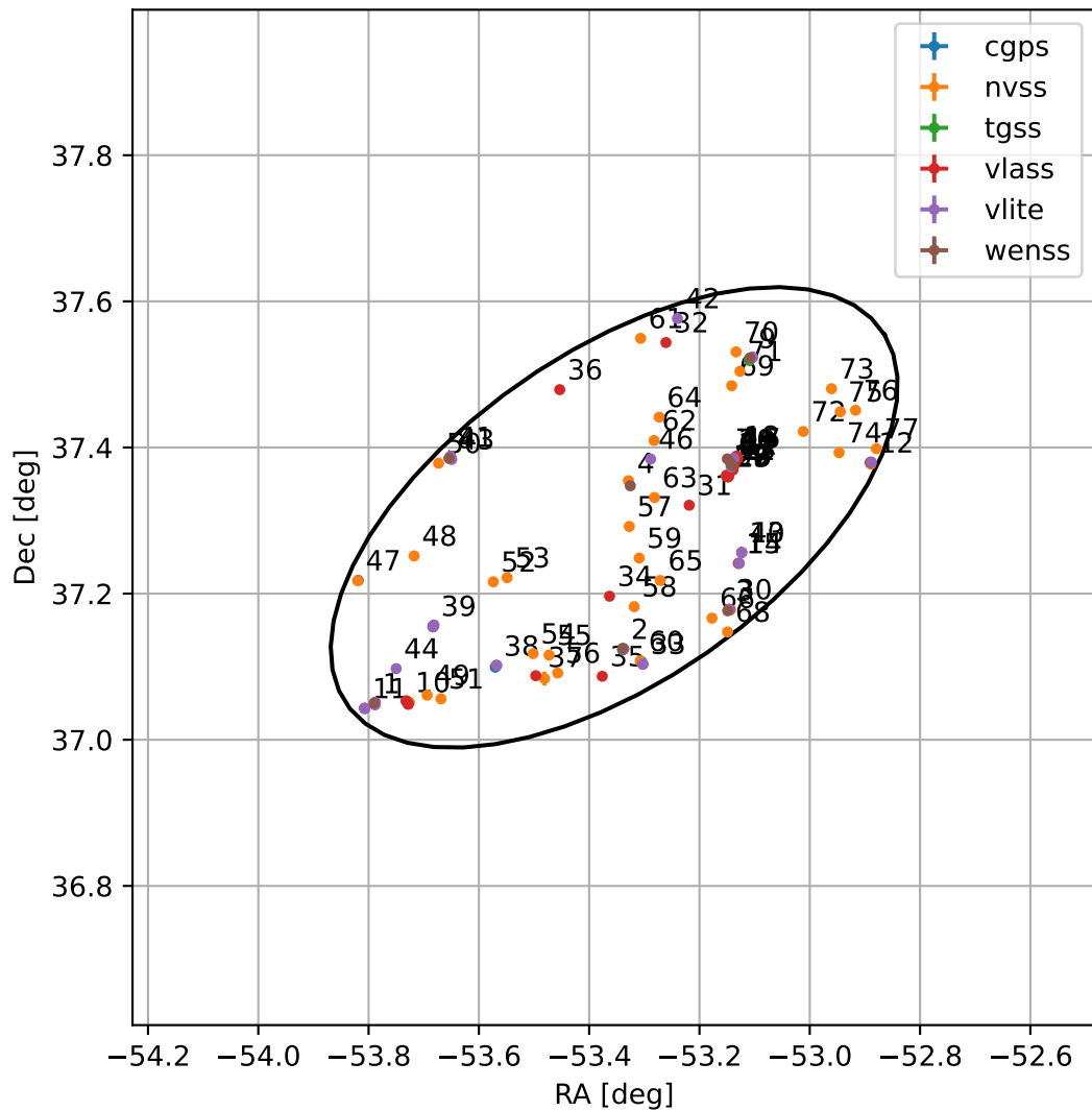
4FGL J2026.5+3718
