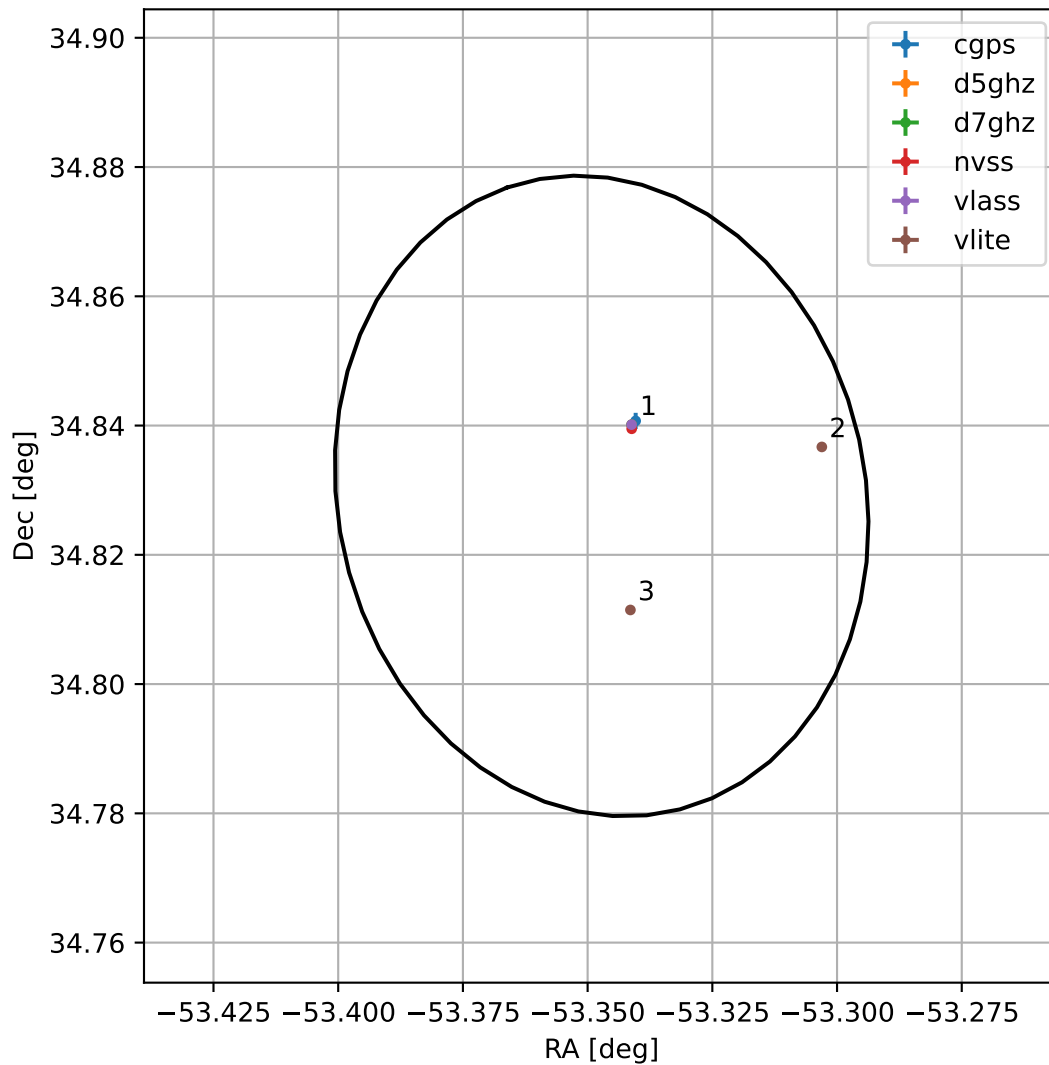
4FGL J2026.6+3449
