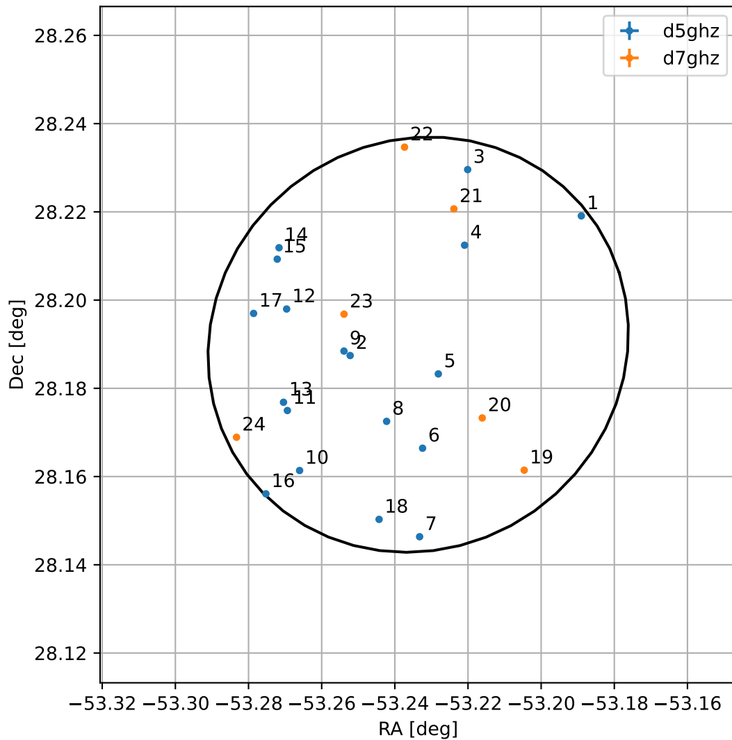
4FGL J2027.0+2811
