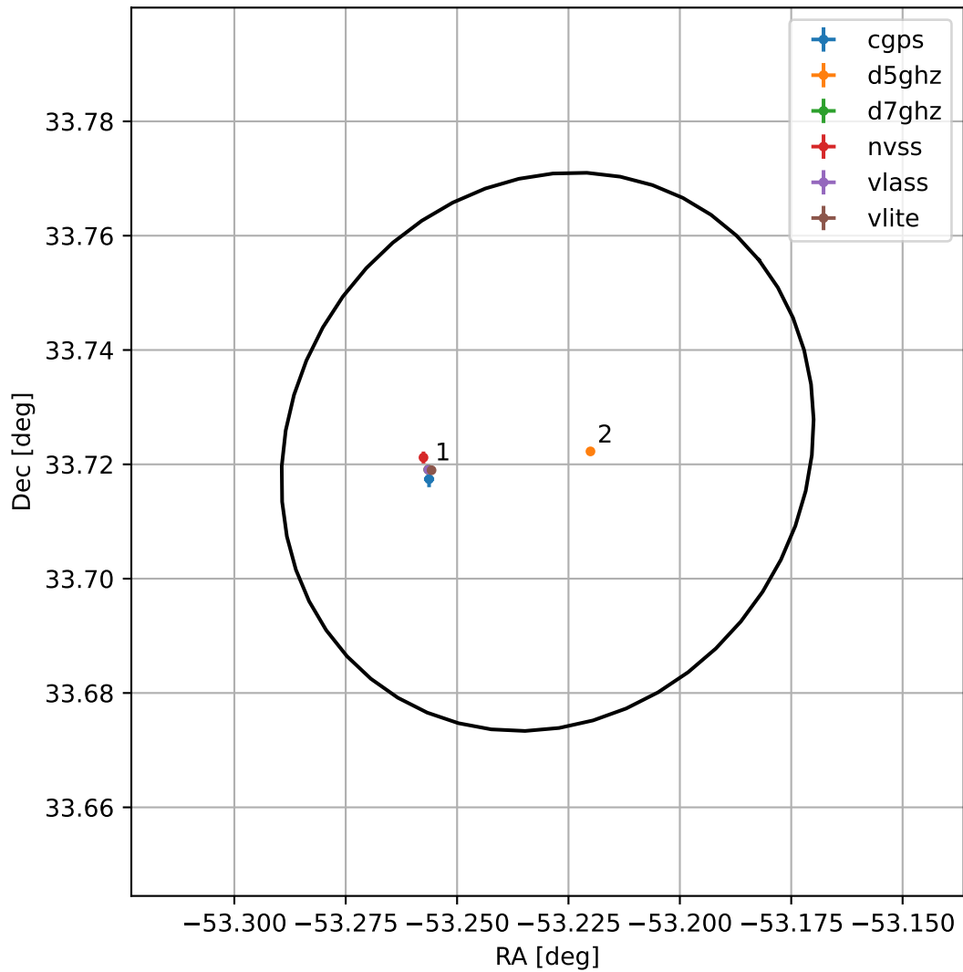
4FGL J2027.0+3343
