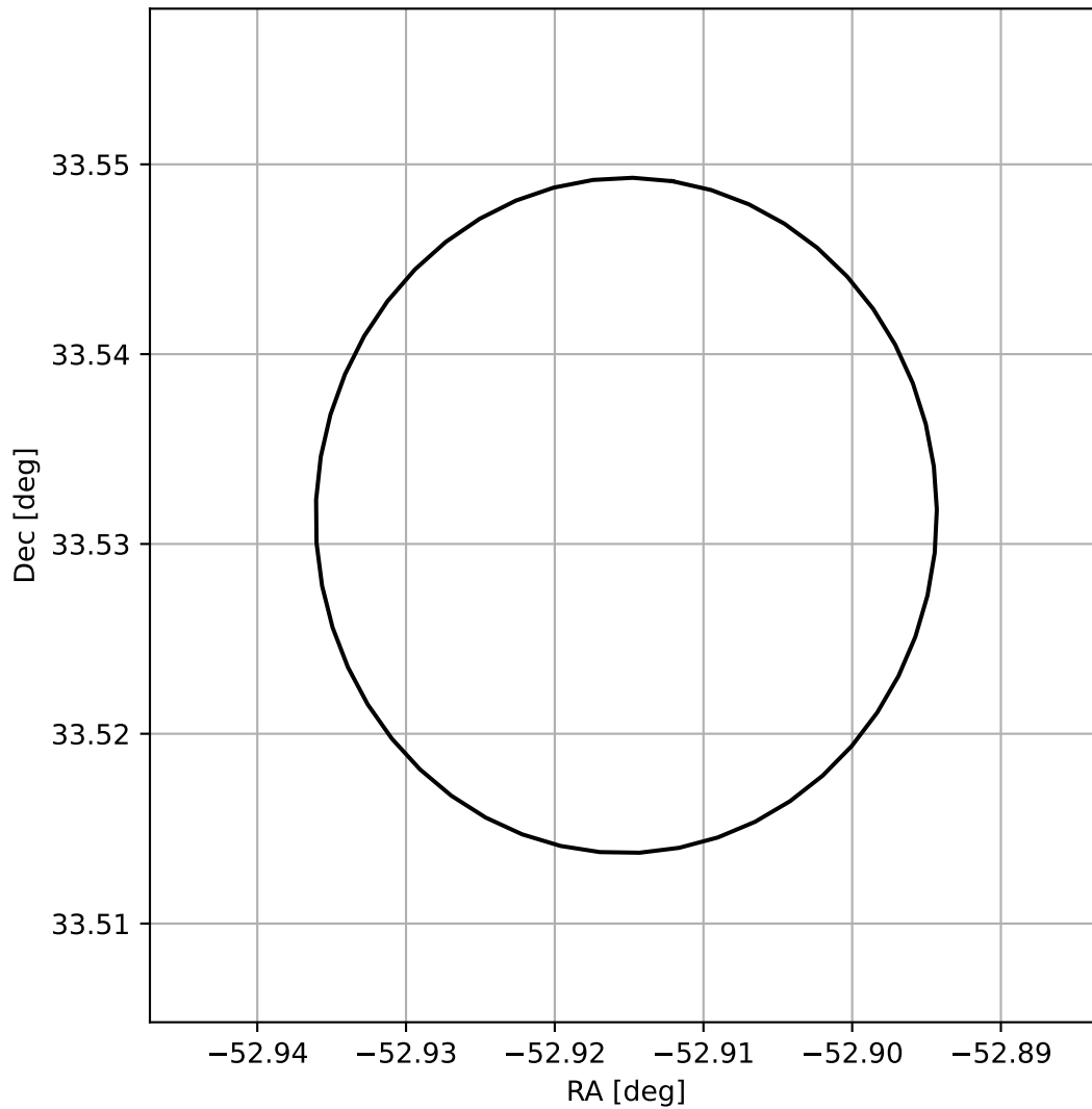
4FGL J2028.3+3331
