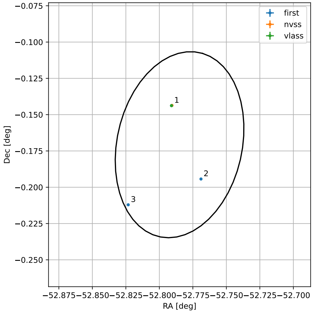
4FGL J2028.8-0010
