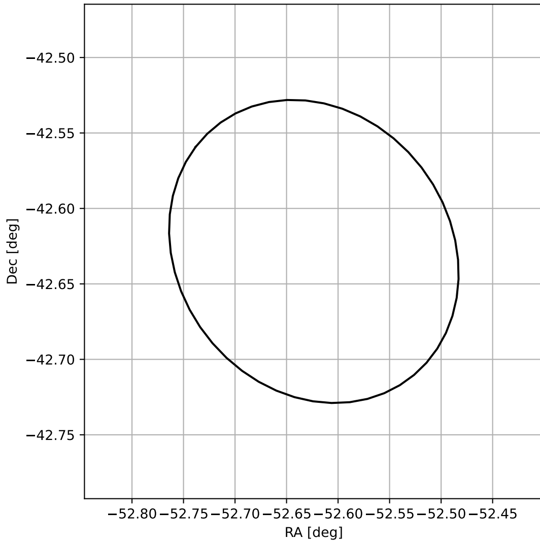
4FGL J2029.5-4237
