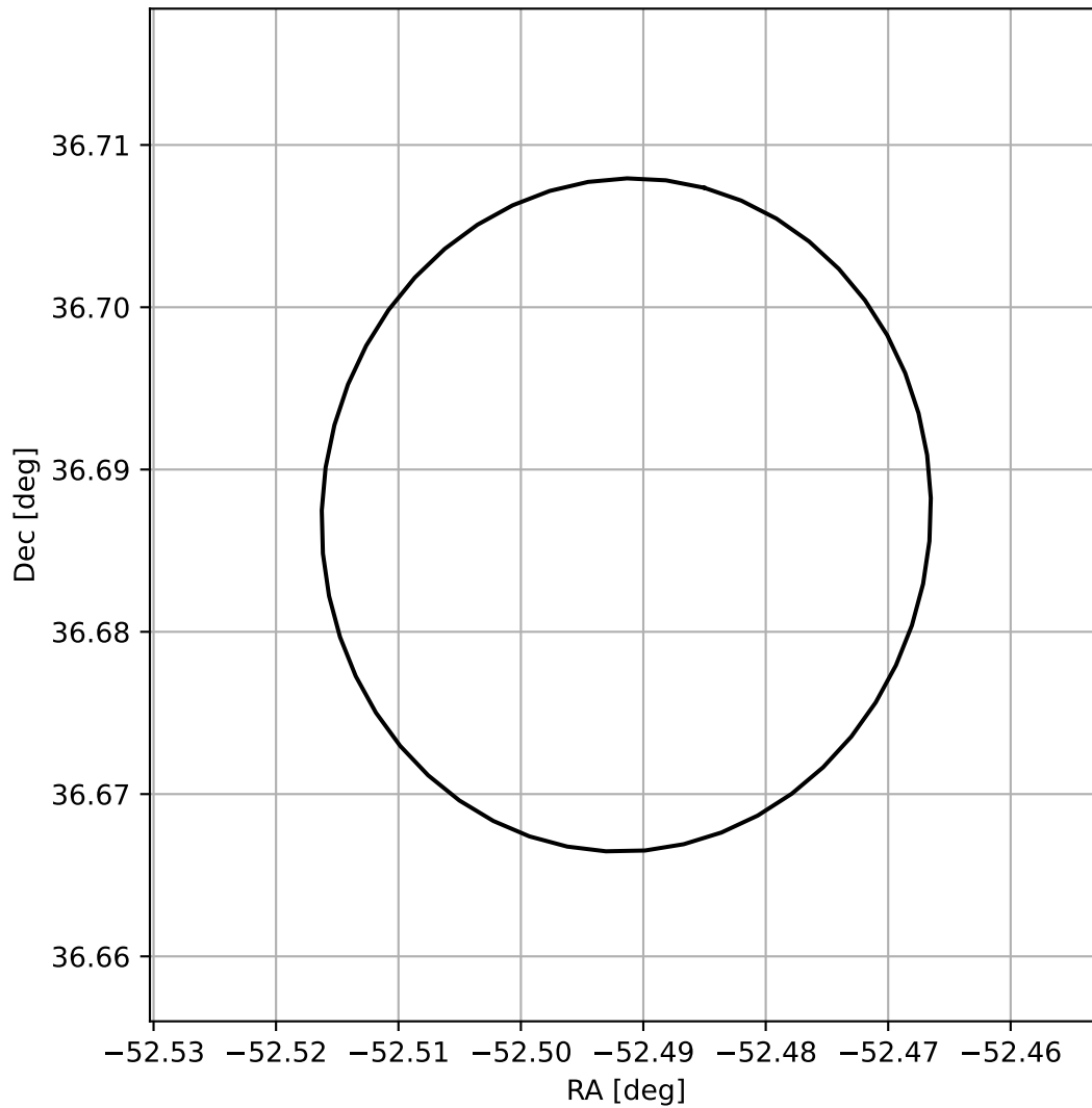
4FGL J2030.0+3641
