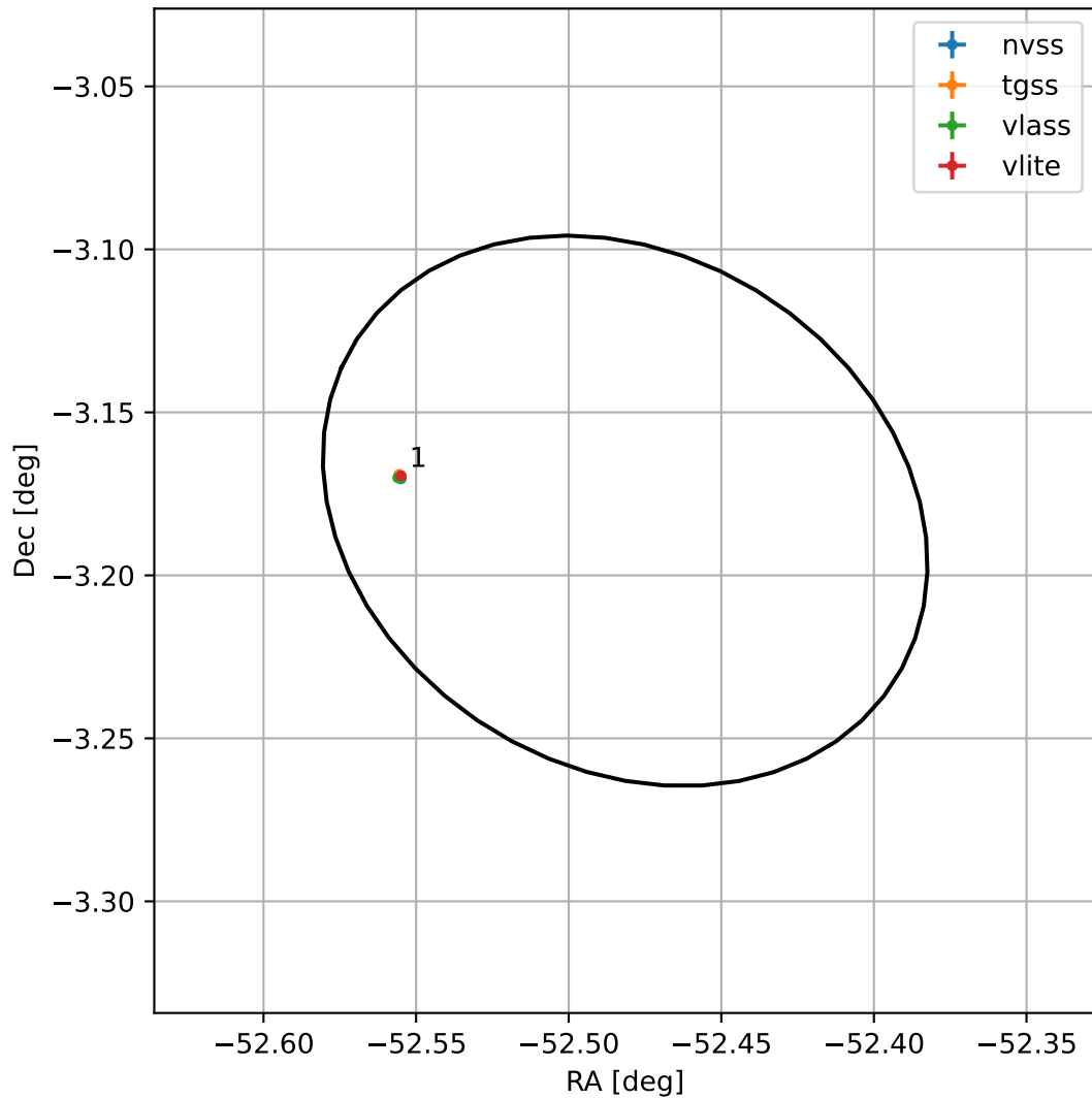
4FGL J2030.0-0310
