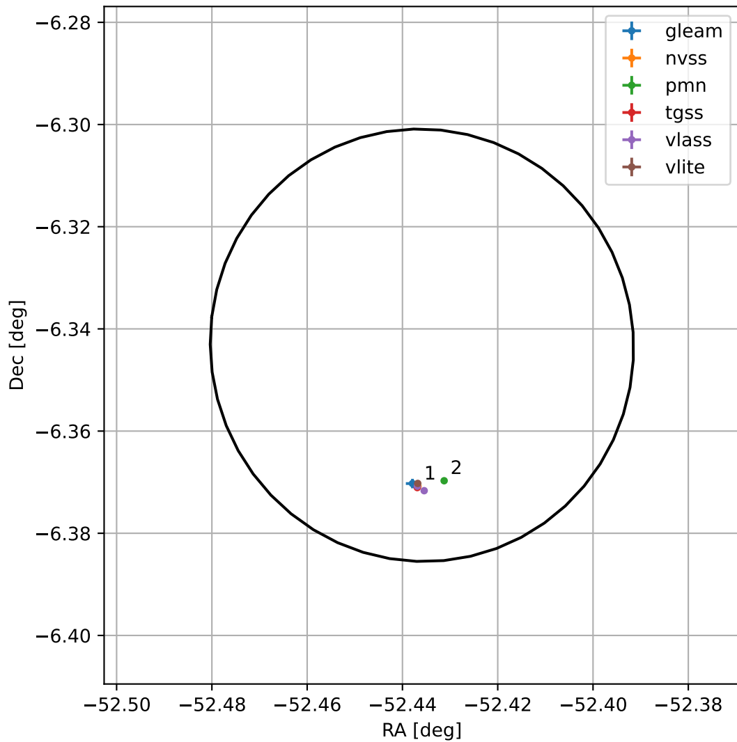
4FGL J2030.2-0620
