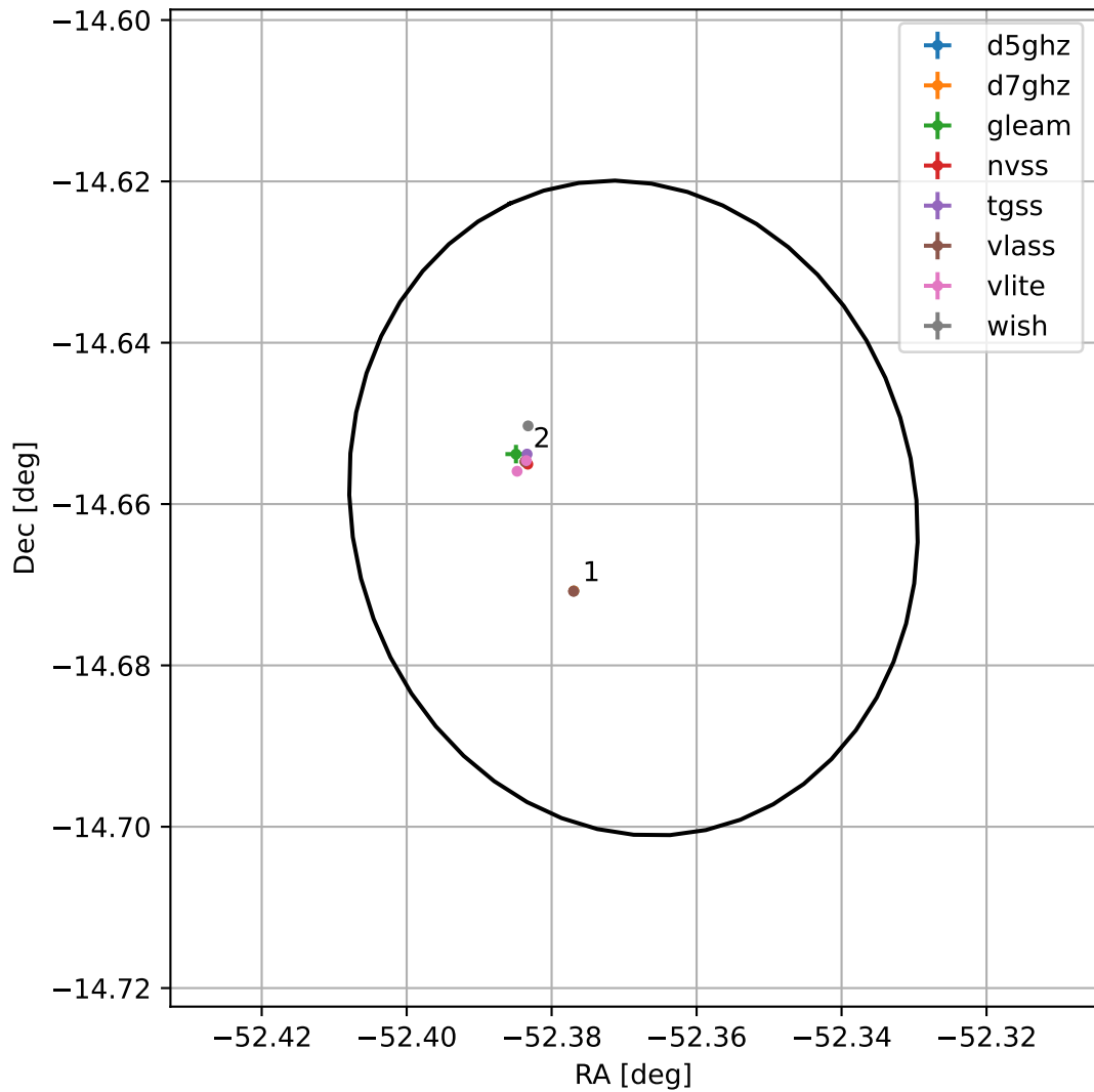
4FGL J2030.5-1439
