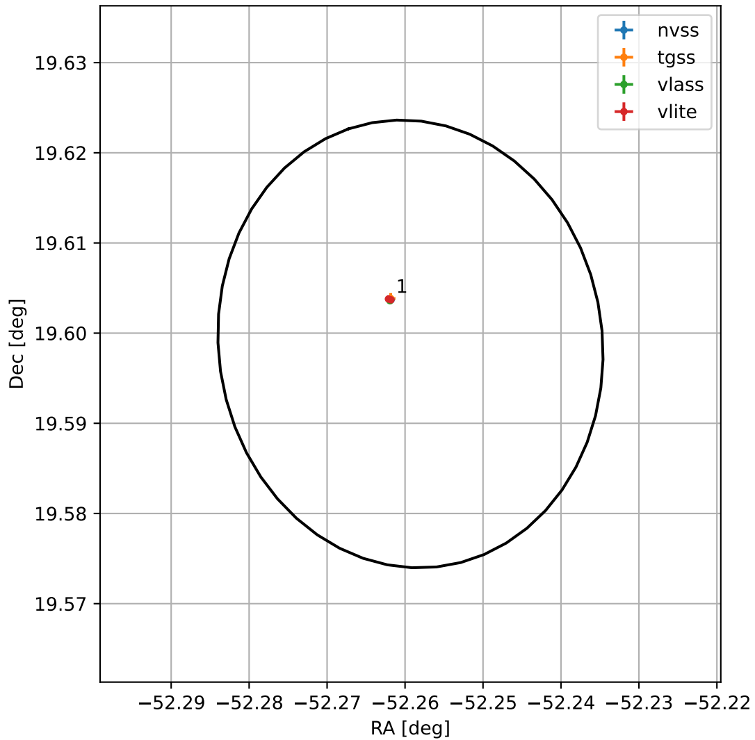
4FGL J2030.9+1935
