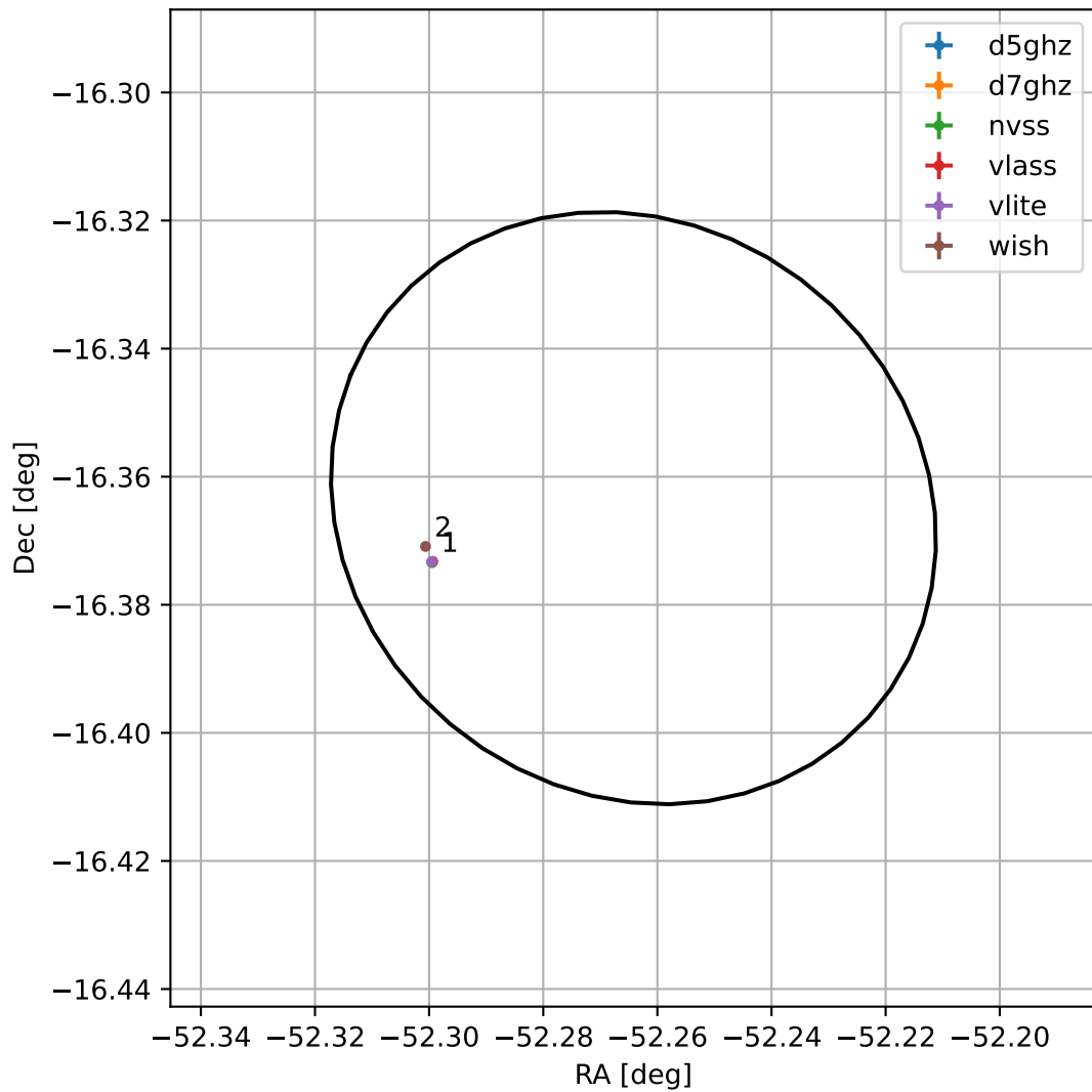
4FGL J2030.9-1621
