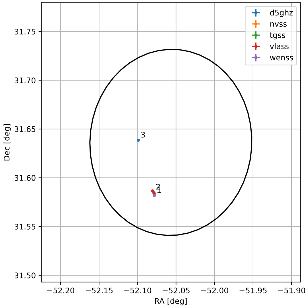
4FGL J2031.7+3138
