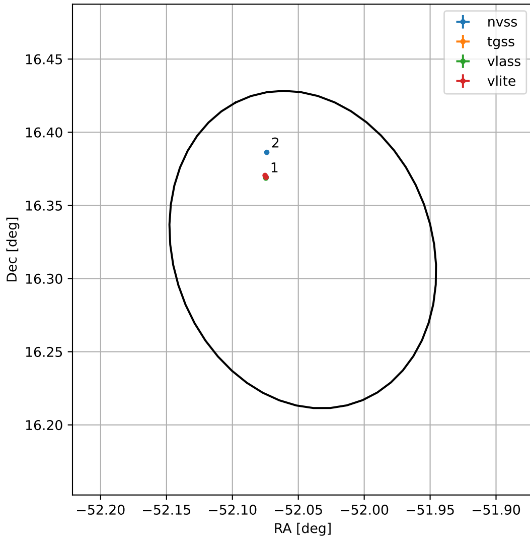
4FGL J2031.8+1619
