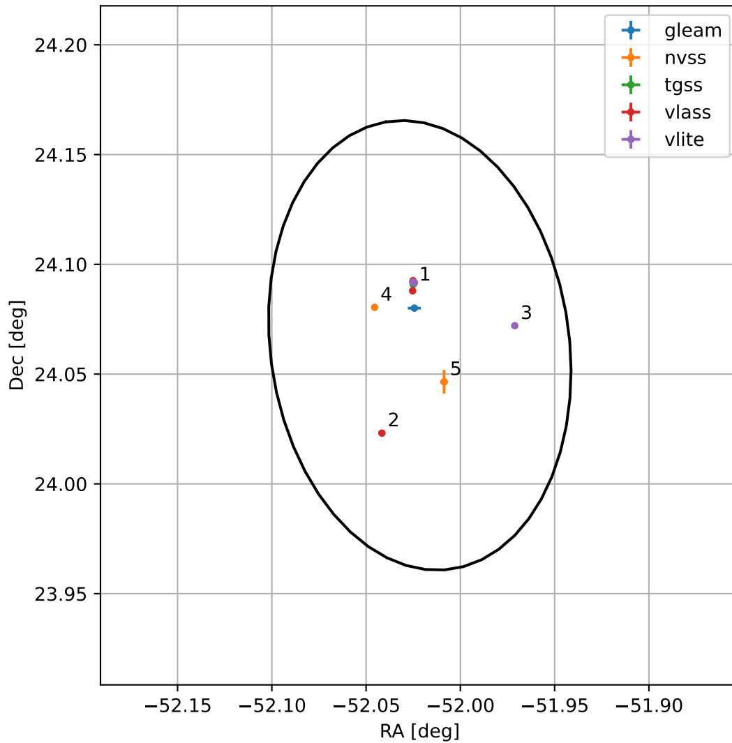
4FGL J2031.9+2403
