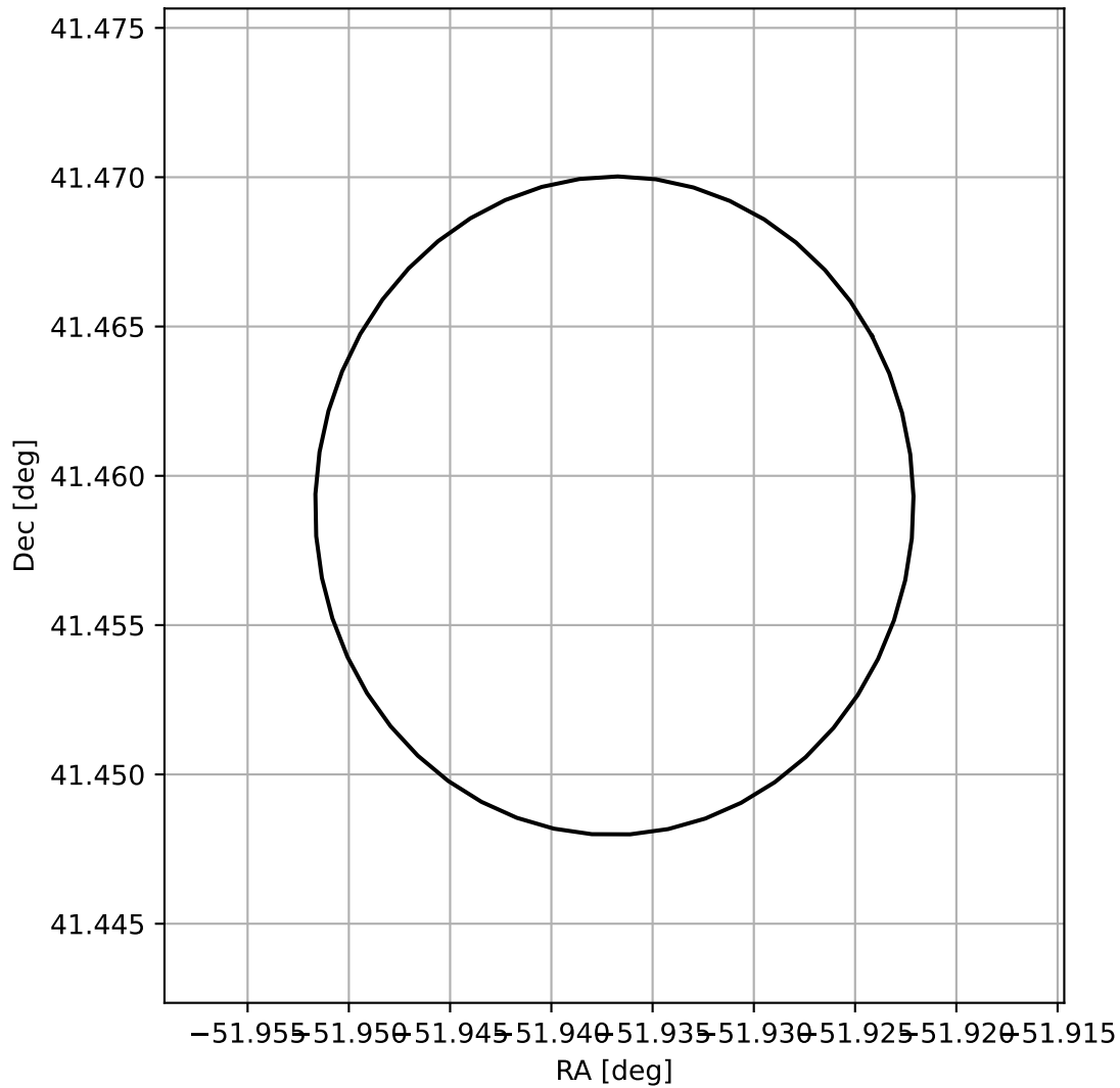
4FGL J2032.2+4127
