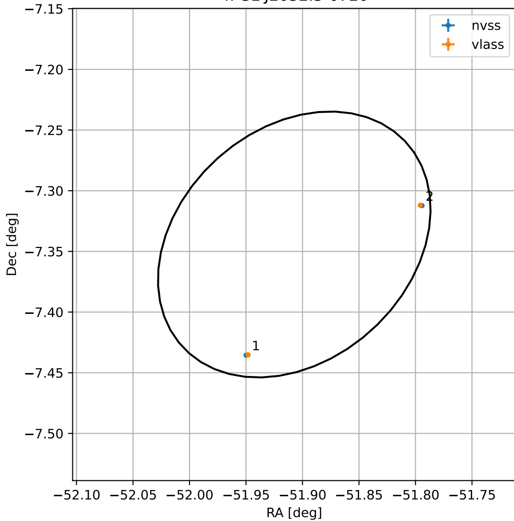
4FGL J2032.3-0720
