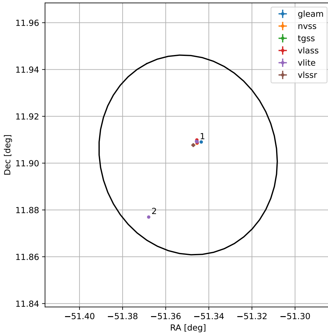
4FGL J2034.6+1154
