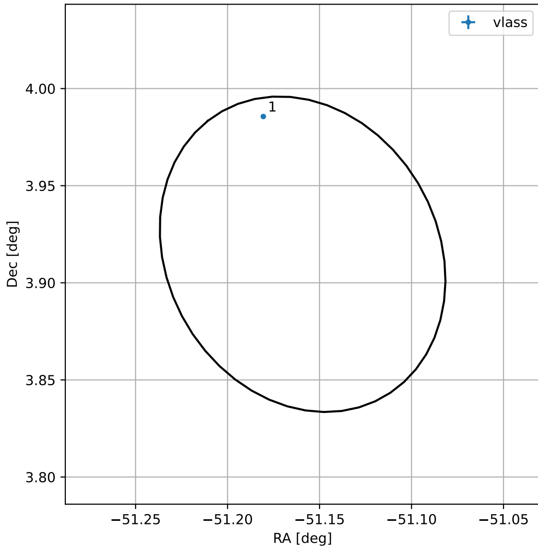
4FGL J2035.3+0354
