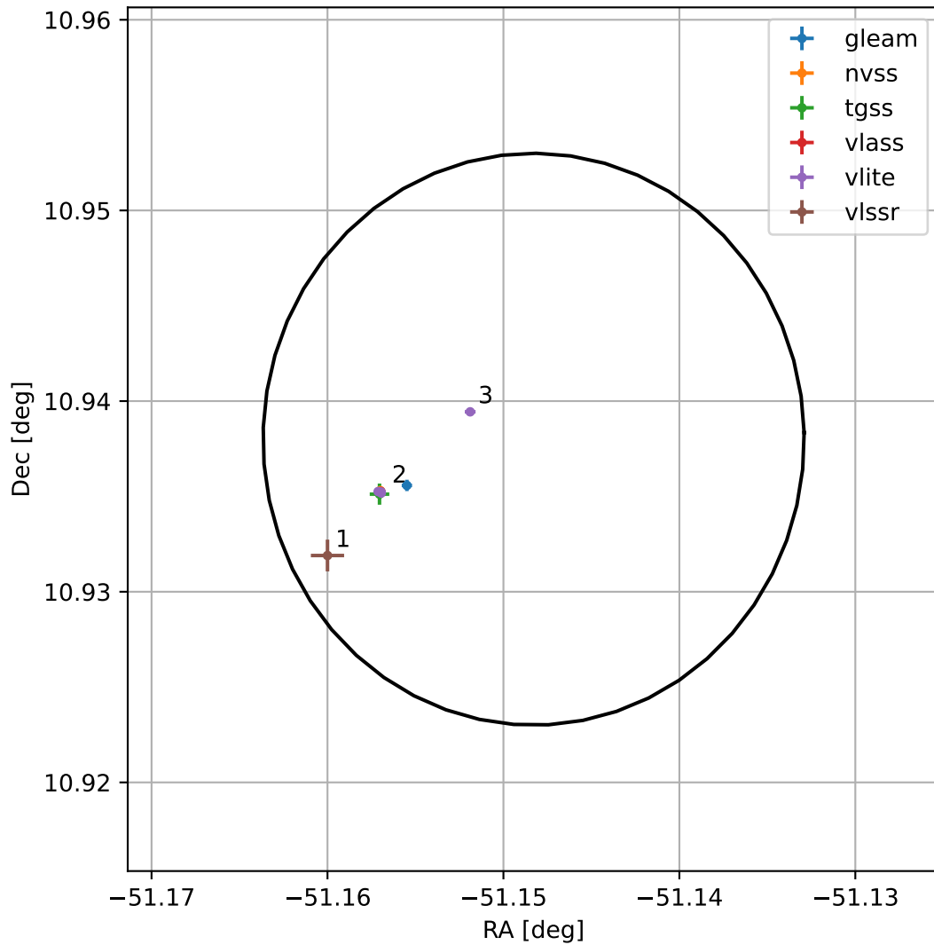
4FGL J2035.4+1056
