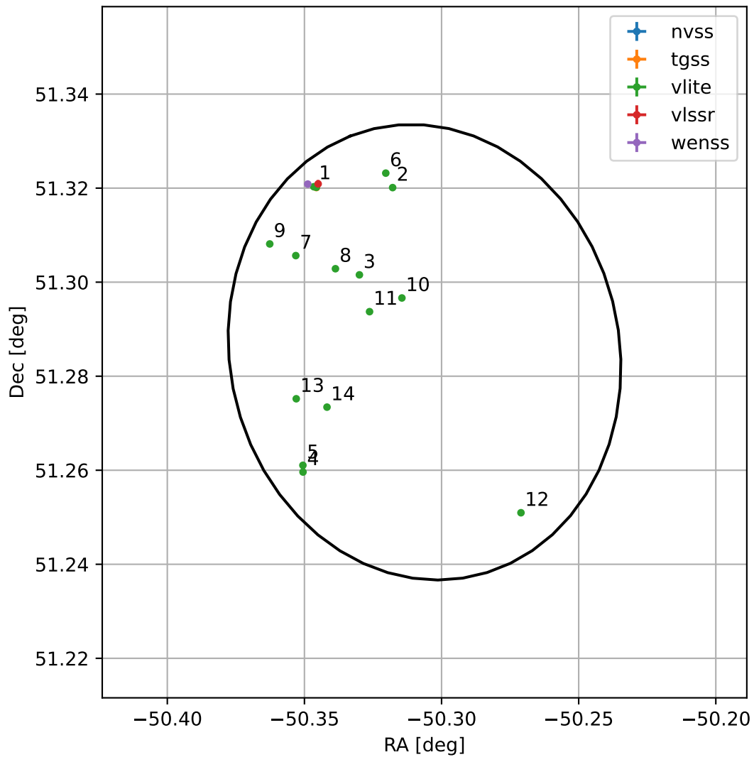
4FGL J2038.7+5117
