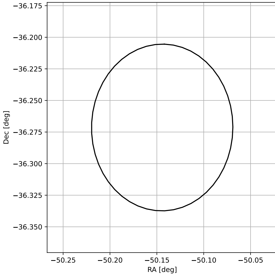
4FGL J2039.4-3616
