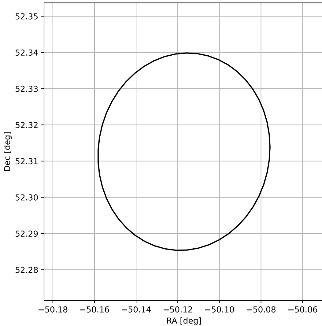
4FGL J2039.5+5218
