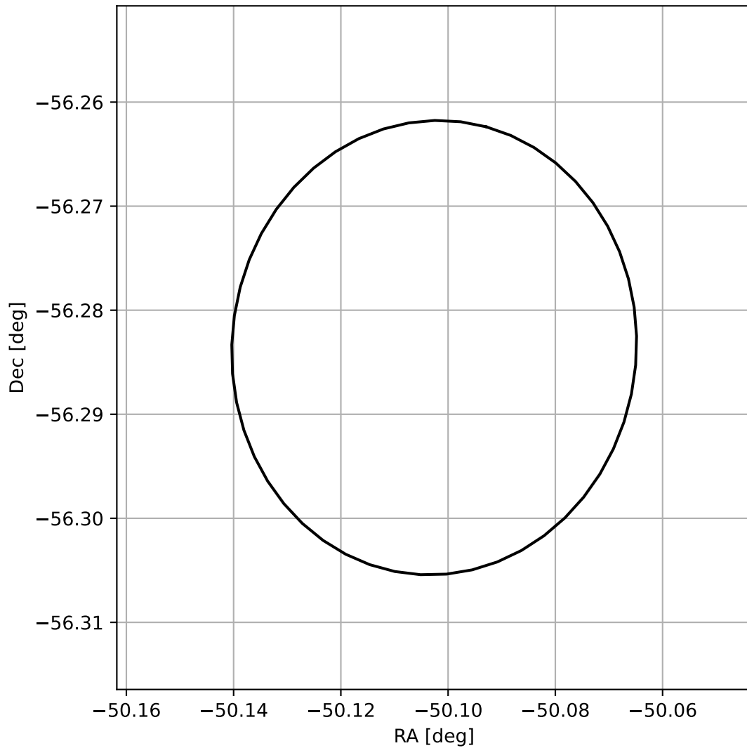
4FGL J2039.5-5617
