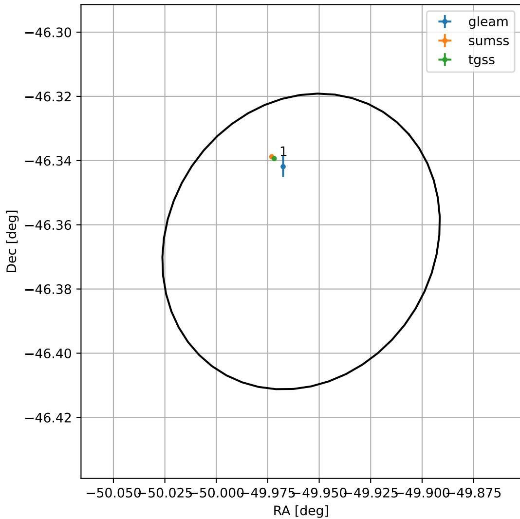
4FGL J2040.1-4621
