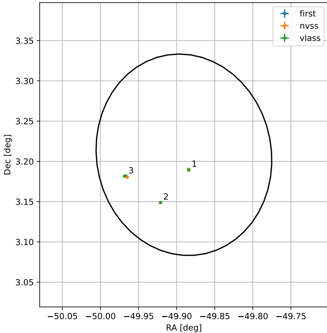
4FGL J2040.4+0312
