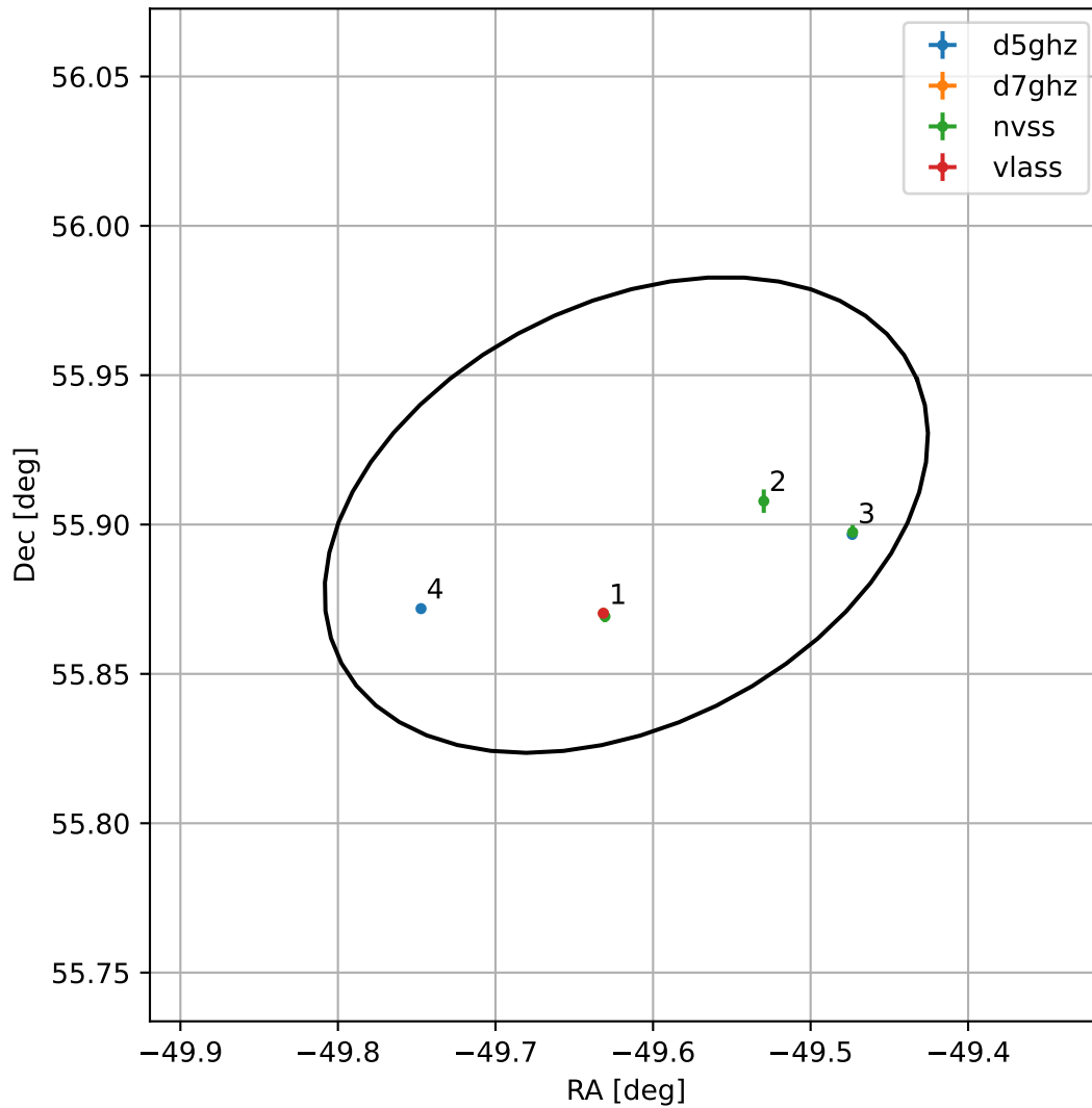
4FGL J2041.5+5554
