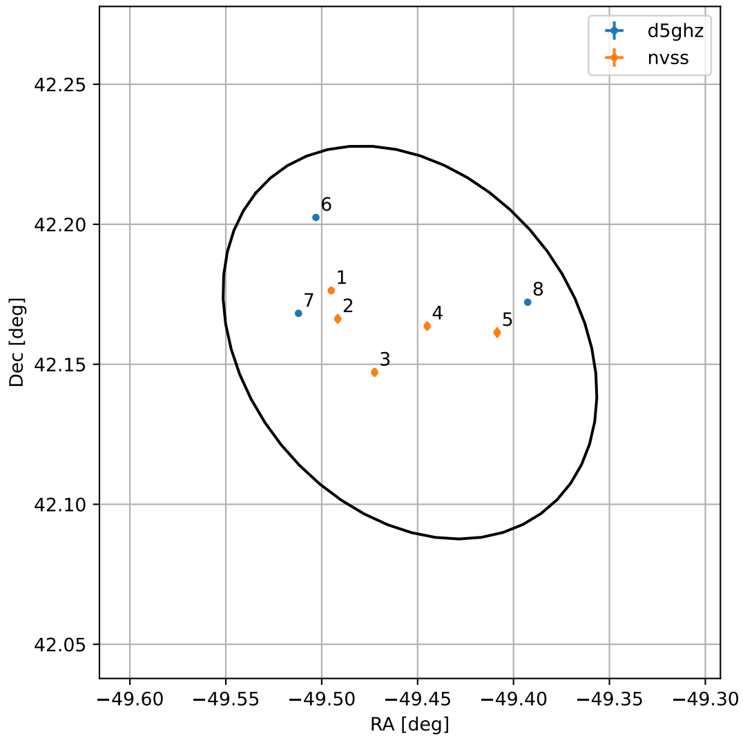
4FGL J2042.1+4209
