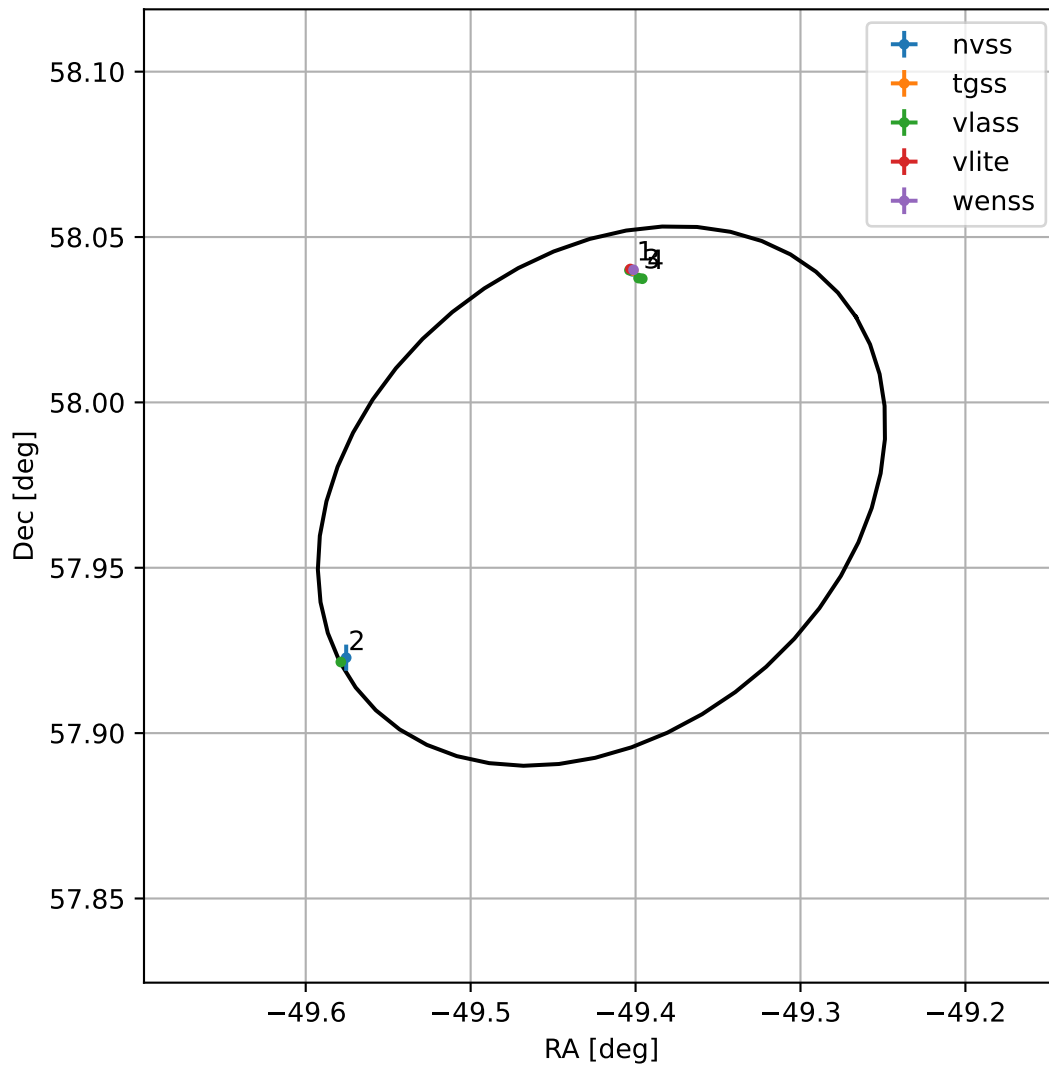
4FGL J2042.3+5758
