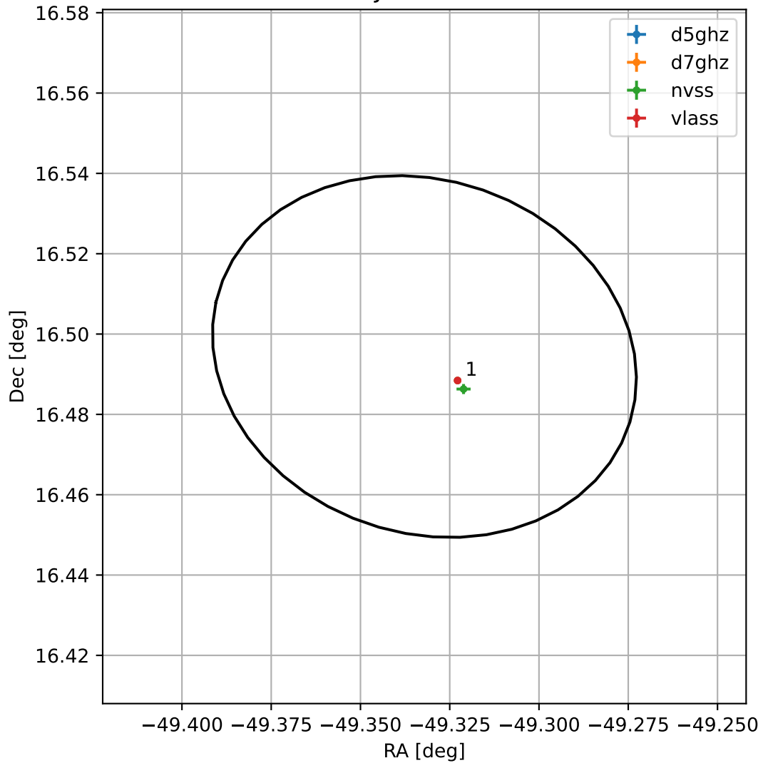
4FGL J2042.6+1629
