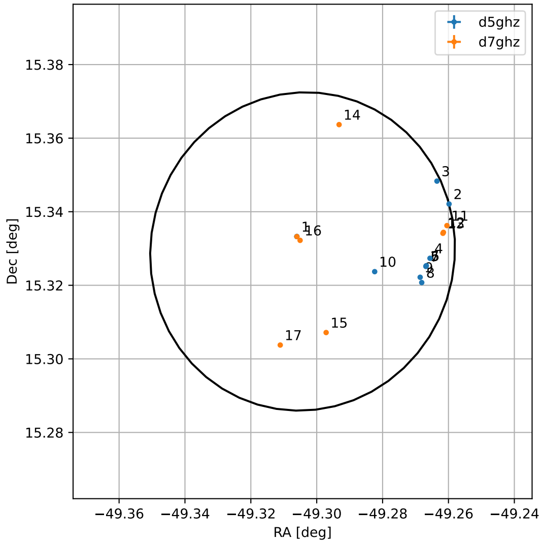
4FGL J2042.7+1519
