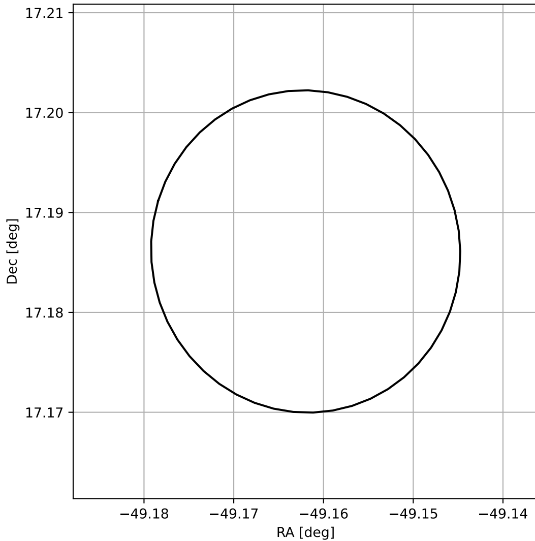
4FGL J2043.3+1711
