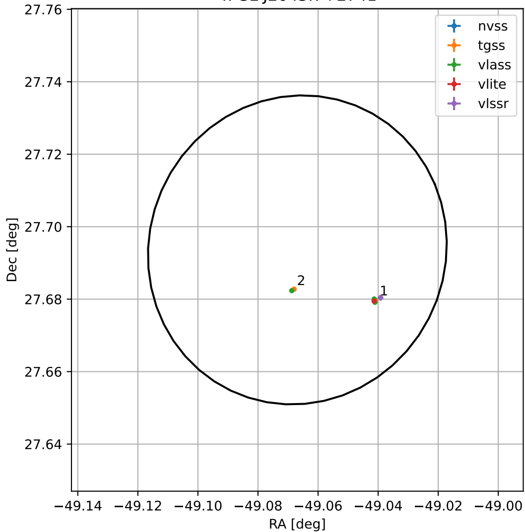
4FGL J2043.7+2741
