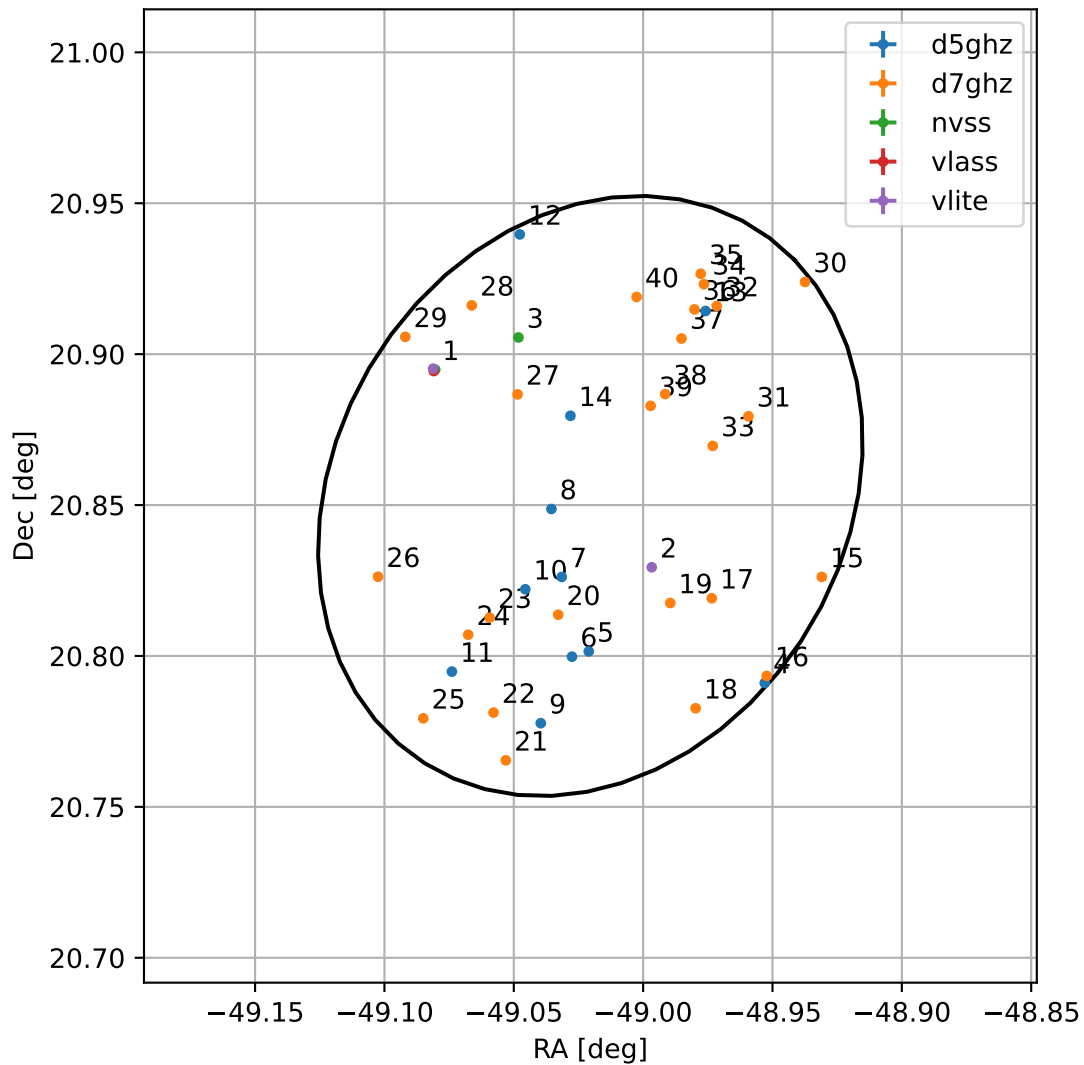
4FGL J2043.9+2051
