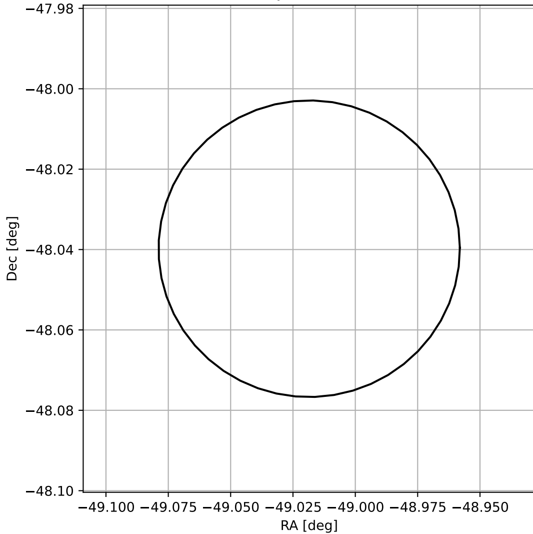
4FGL J2043.9-4802
