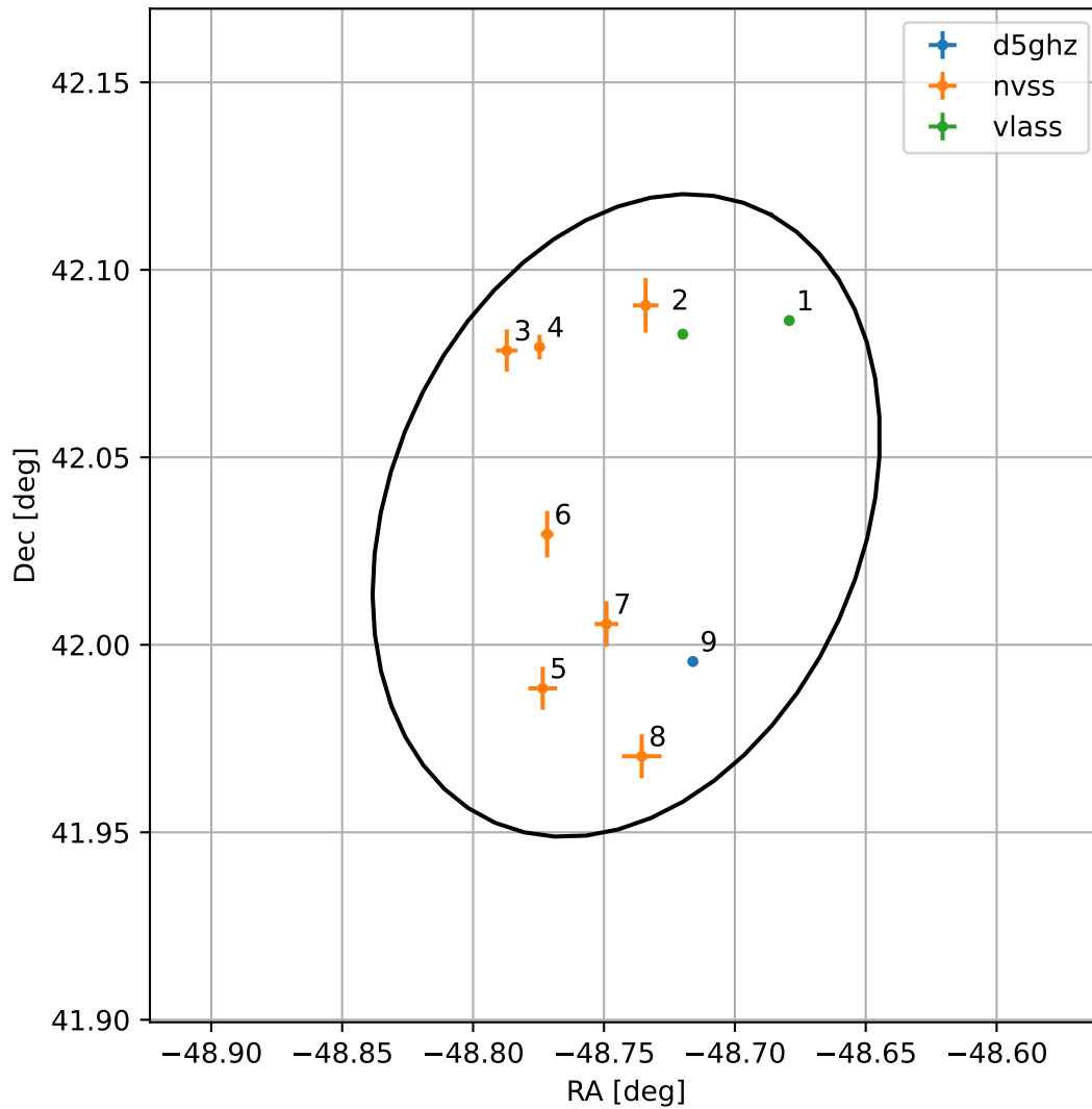
4FGL J2045.0+4202
