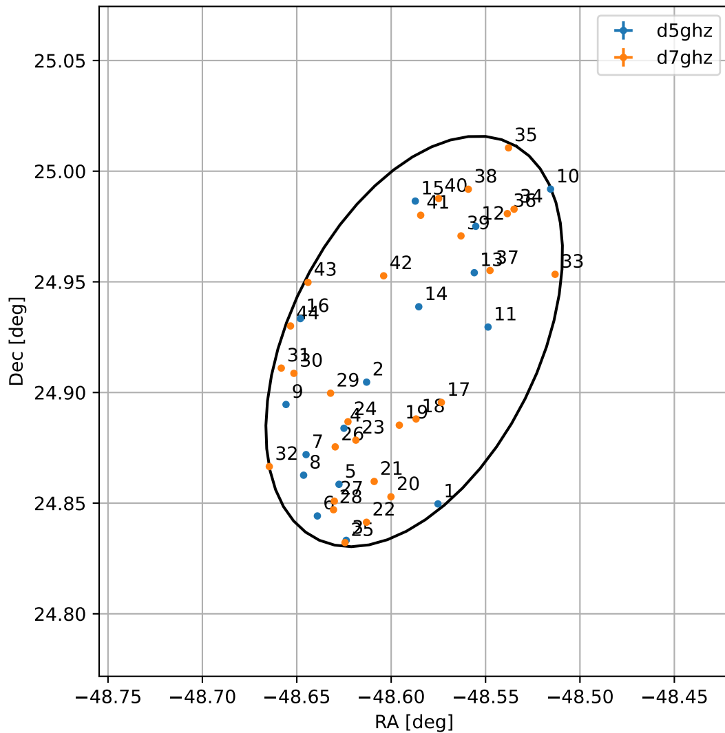
4FGL J2045.6+2455
