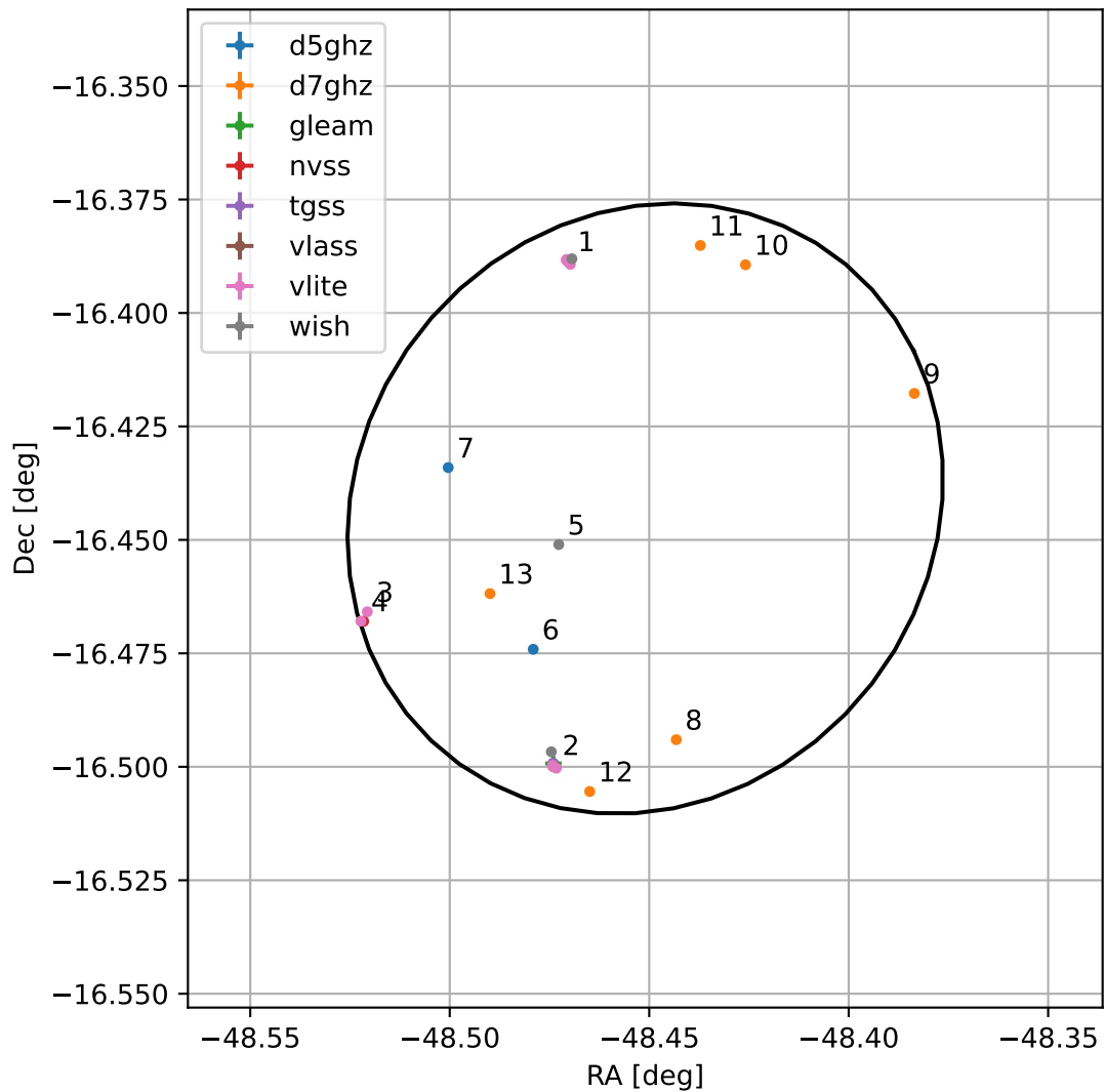
4FGL J2046.1-1626
