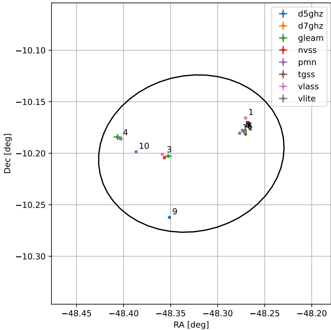
4FGL J2046.6-1012
