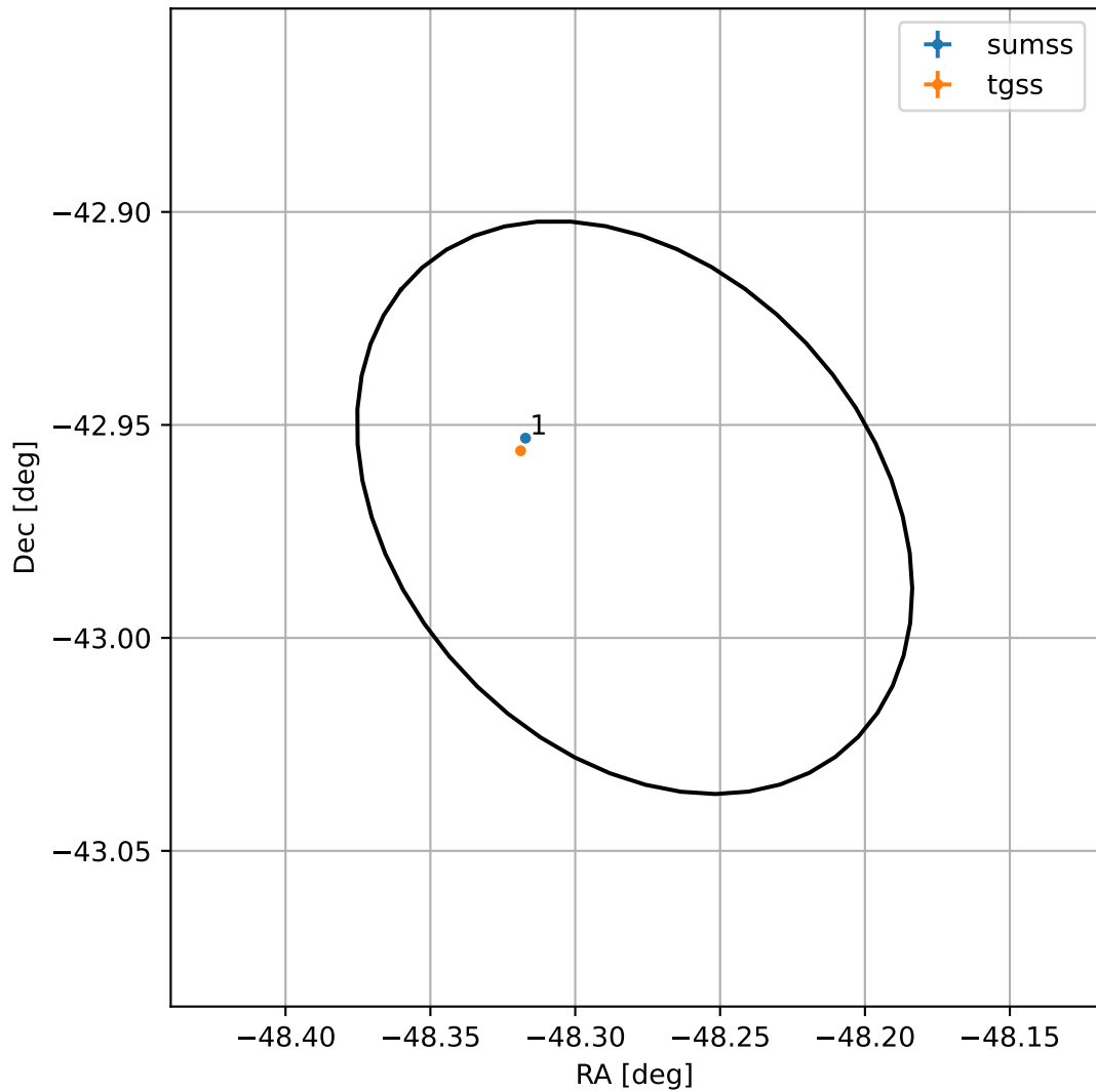
4FGL J2046.8-4258
