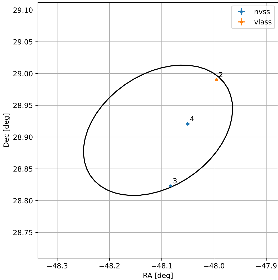
4FGL J2047.5+2854
