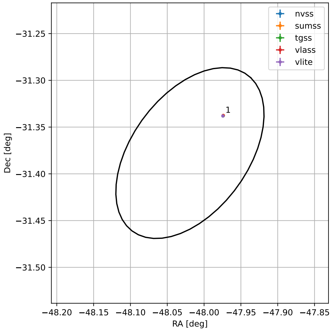
4FGL J2047.9-3122
