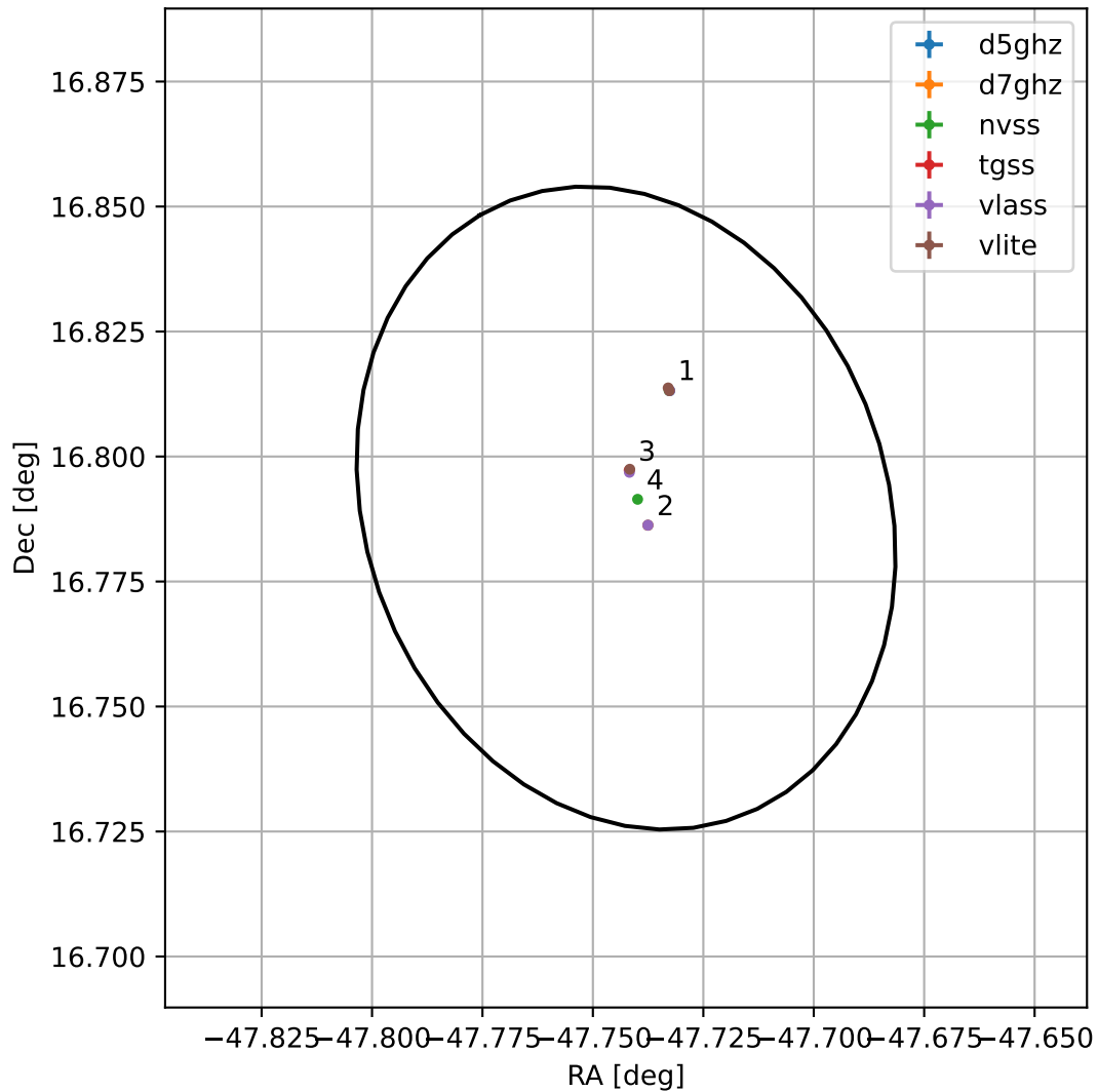
4FGL J2049.0+1647
