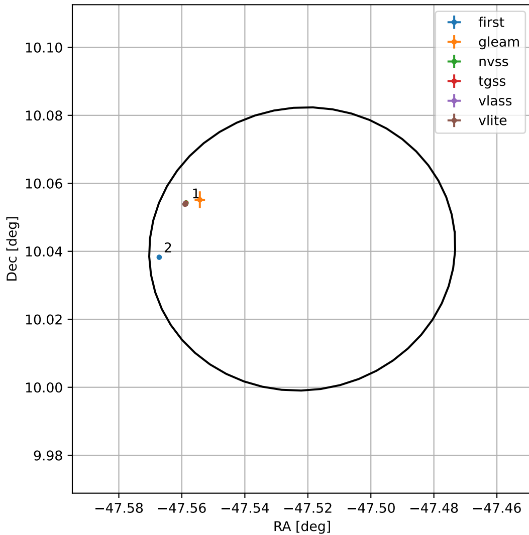
4FGL J2049.9+1002
