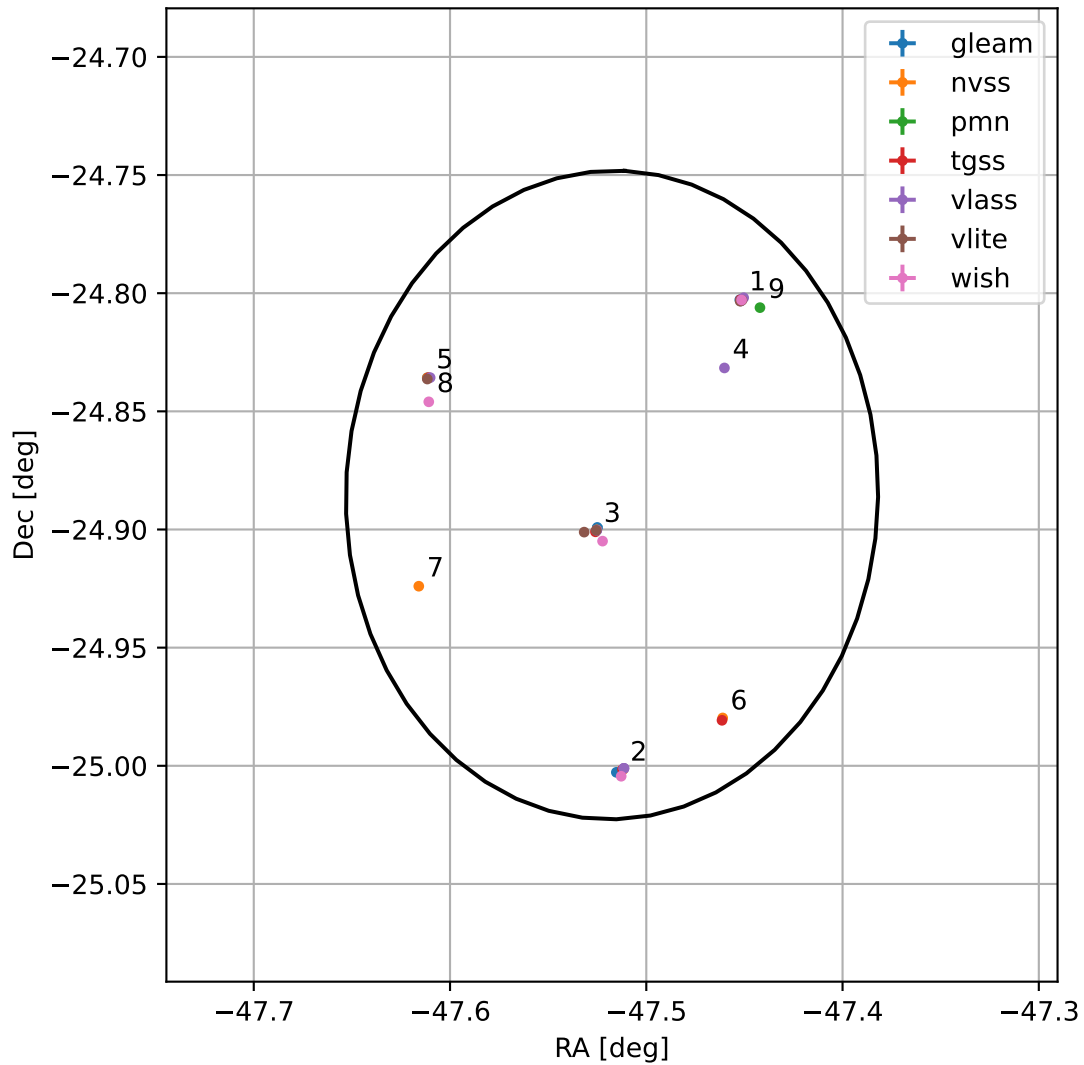
4FGL J2049.9-2453
